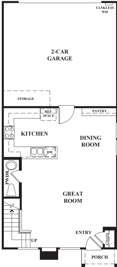
LEVEL 1
